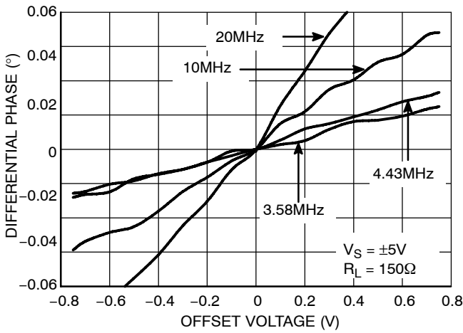
Figure 17. Differential Phase
